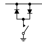
Figure 28. Line Clamp
