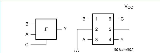
Figure 8. 2-input MUX
