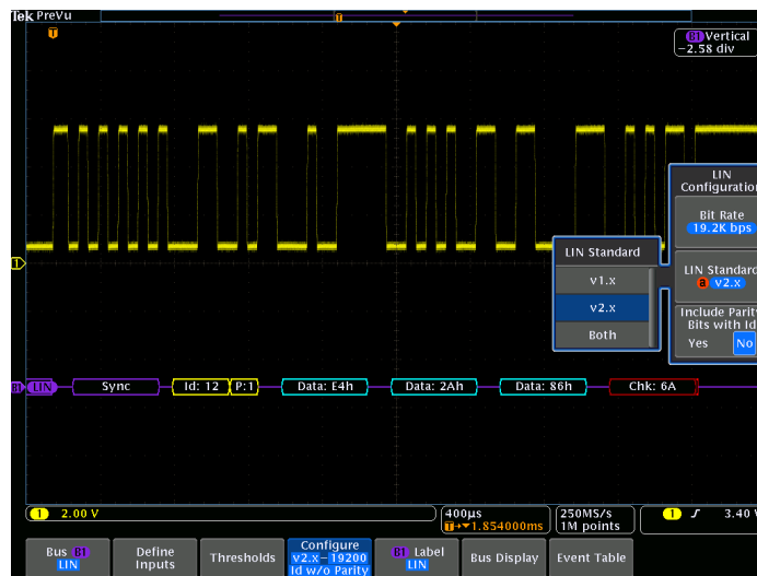
LIN bus setup, showing source configuration options for LIN bus.
