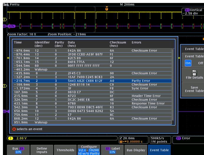
Event table for LIN bus with all captured packets time stamped and in a tabular view.
