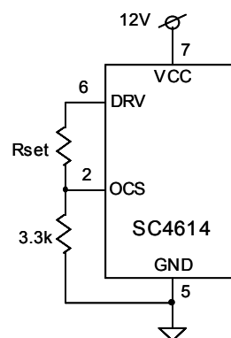
Fig. 1. Programming load trip point
