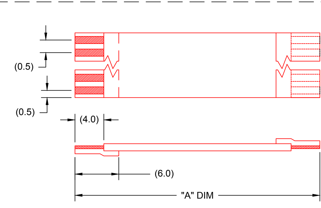
TYPE "D"
