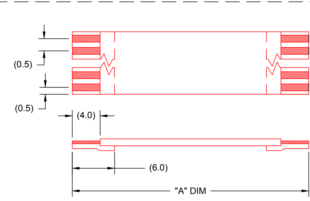
TYPE "A"
