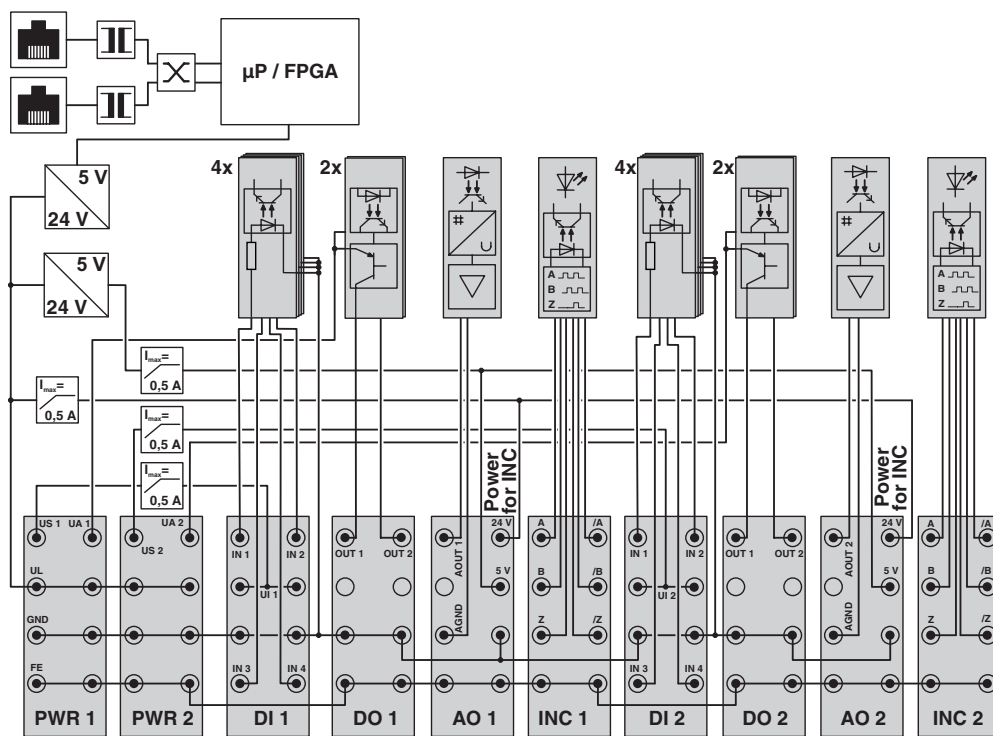
Figure 2 Internal wiring of the terminal points
