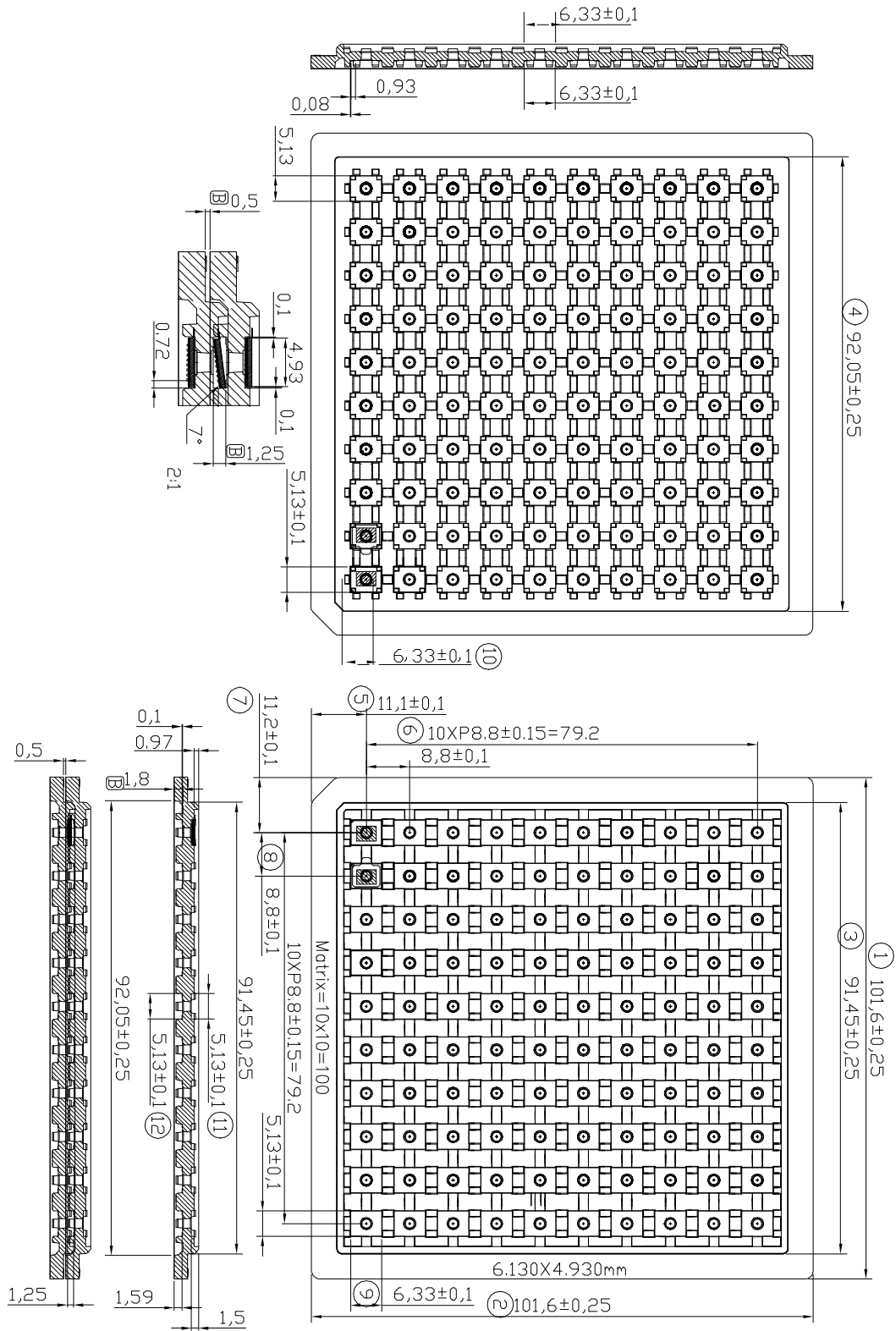
Figure 45. Tray Drawing
