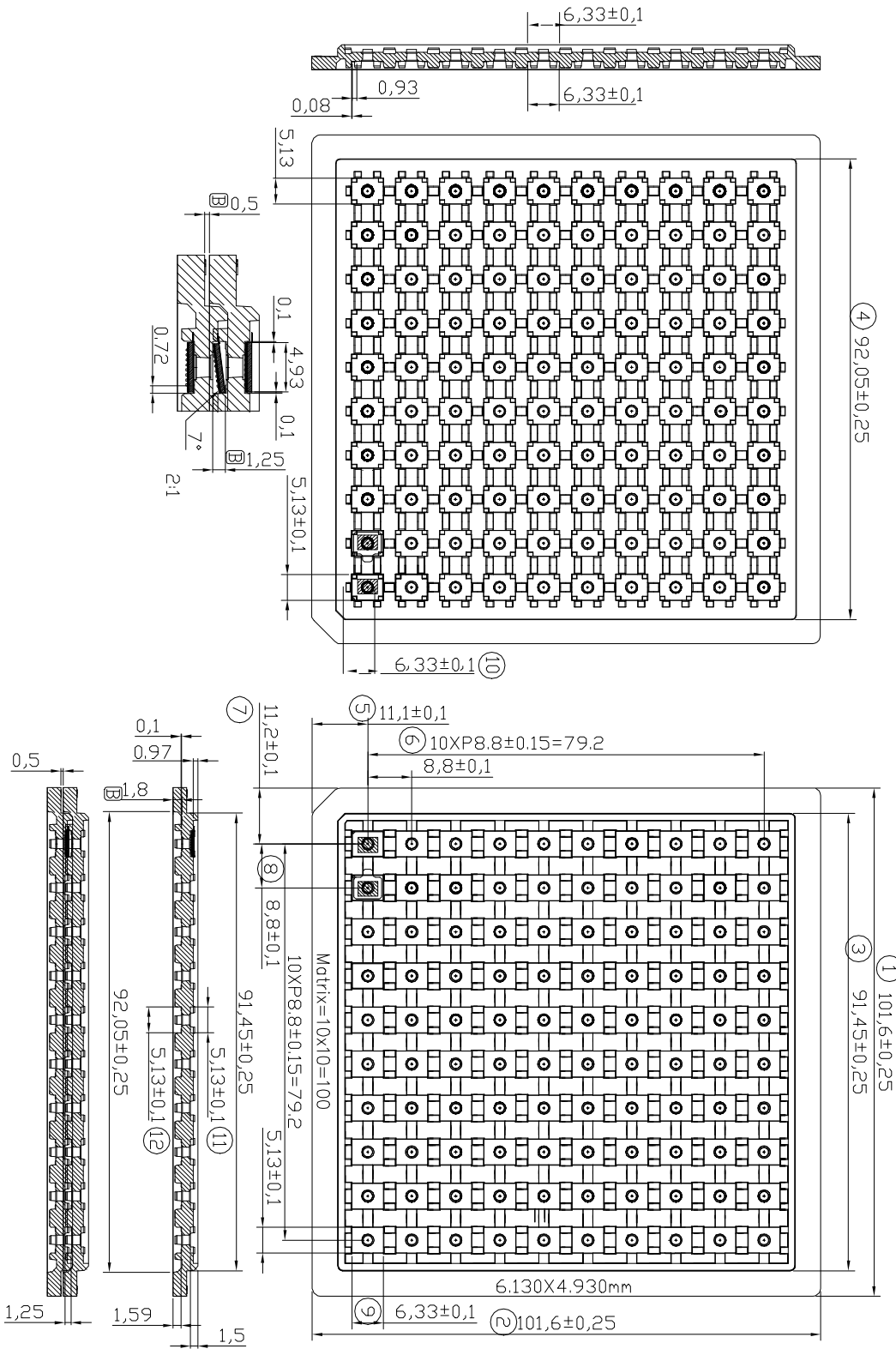
Figure 45. Tray Drawing
