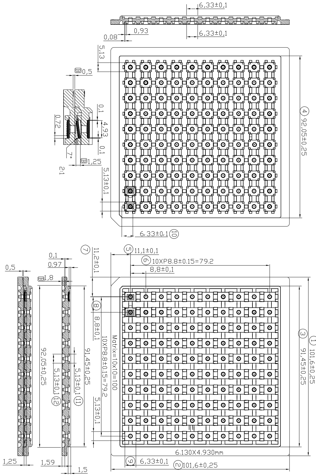
Figure 45. Tray Drawing
