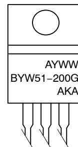
TO-220AB CASE 221A PLASTIC
