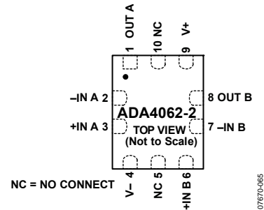
Figure 2. 10-Lead LFCSP
