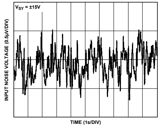
Figure 51. 0.1 Hz to 10 Hz Noise
