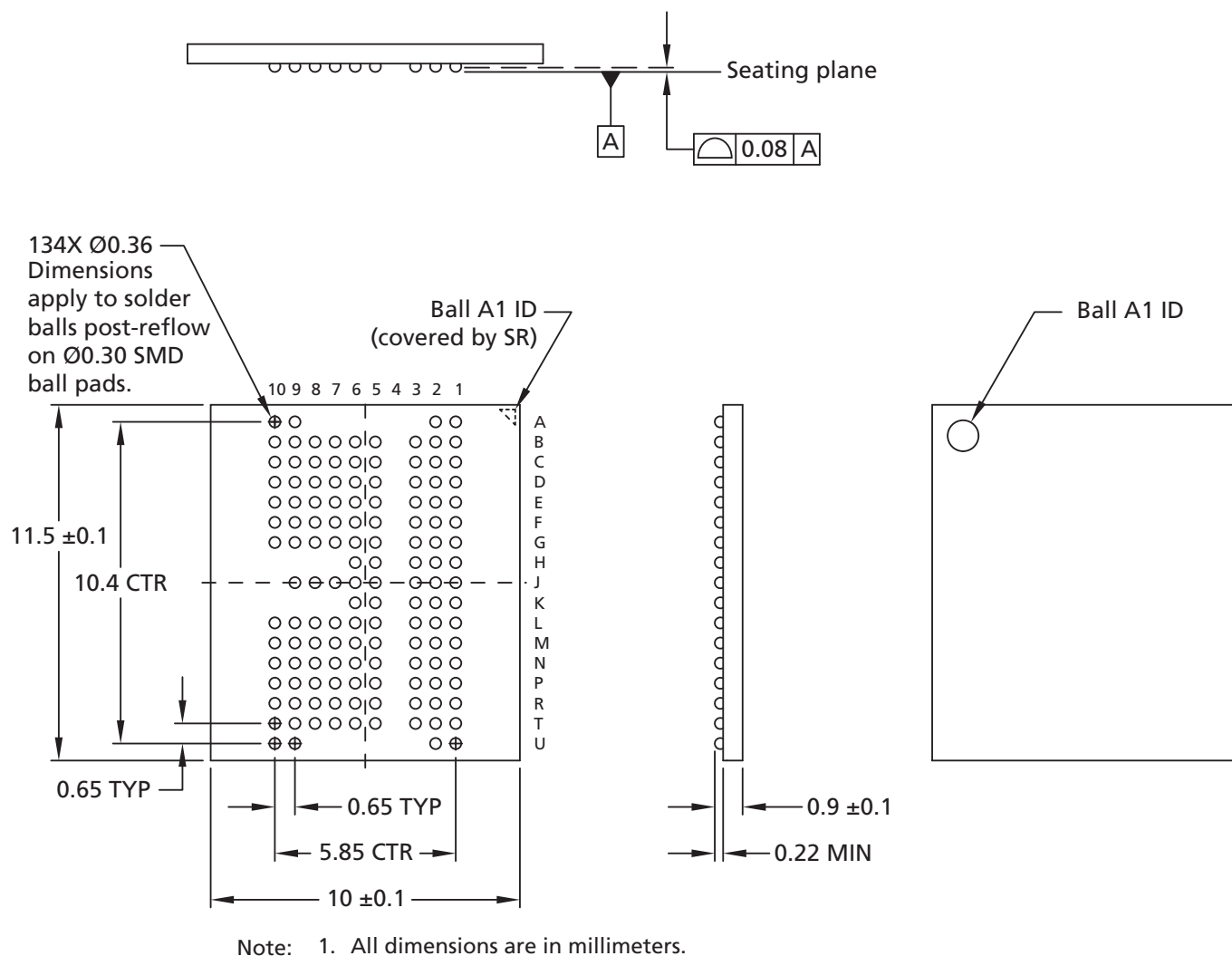
Figure 7: 134-Ball VFBGA – 10mm x 11.5mm (Package Code: BH, MA)
