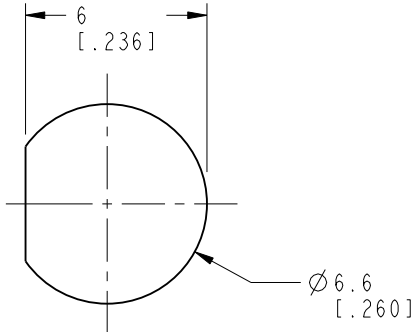
RECOMMENDED PANEL CUTOUT DIMENSIONS
