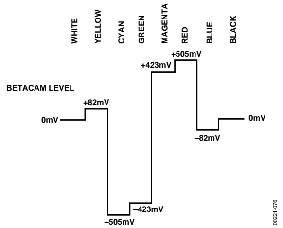
Figure 76. NTSC 100% Color Bars, No Pedestal V Levels
