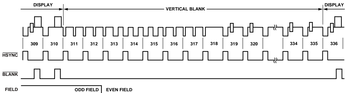
Figure 32. Timing Mode 3 (PAL)
