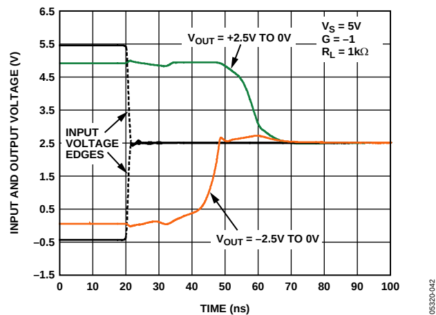
Figure 40. Overload Recovery
