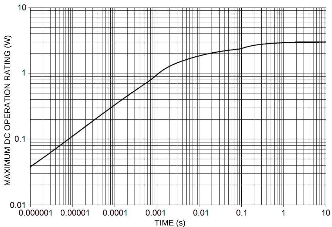
FIGURE 2 Thermal Impedance
