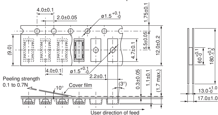
Dimensions of Carrier Tape
