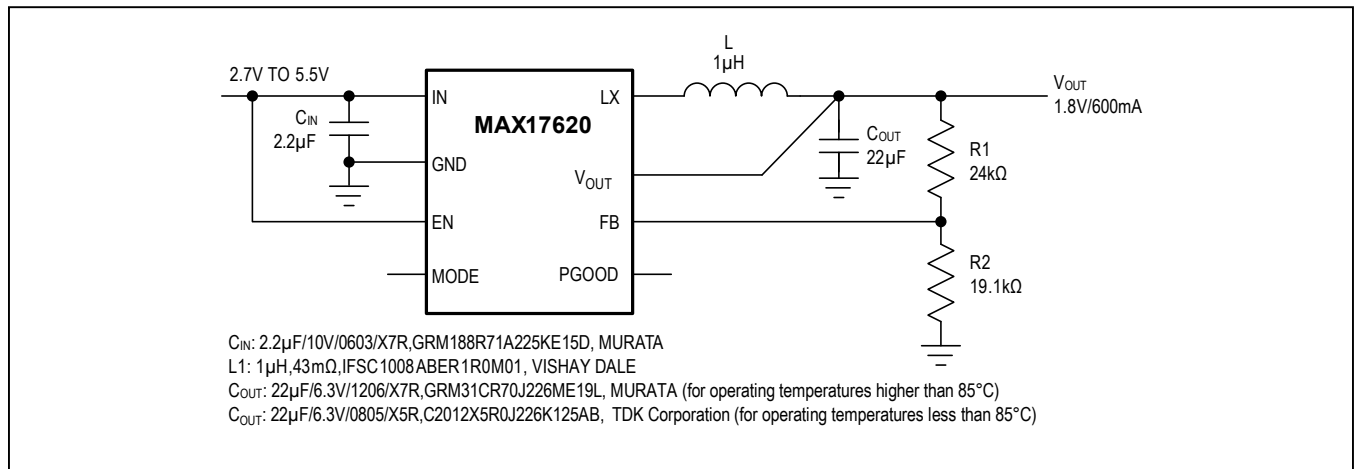
Figure 2. 1.8V, 600mA Step-Down Regulator
