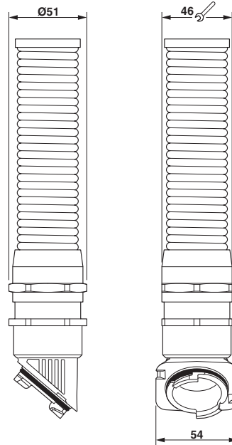
Dimensional drawing
