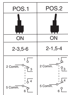
SWITCH FUNCTION
