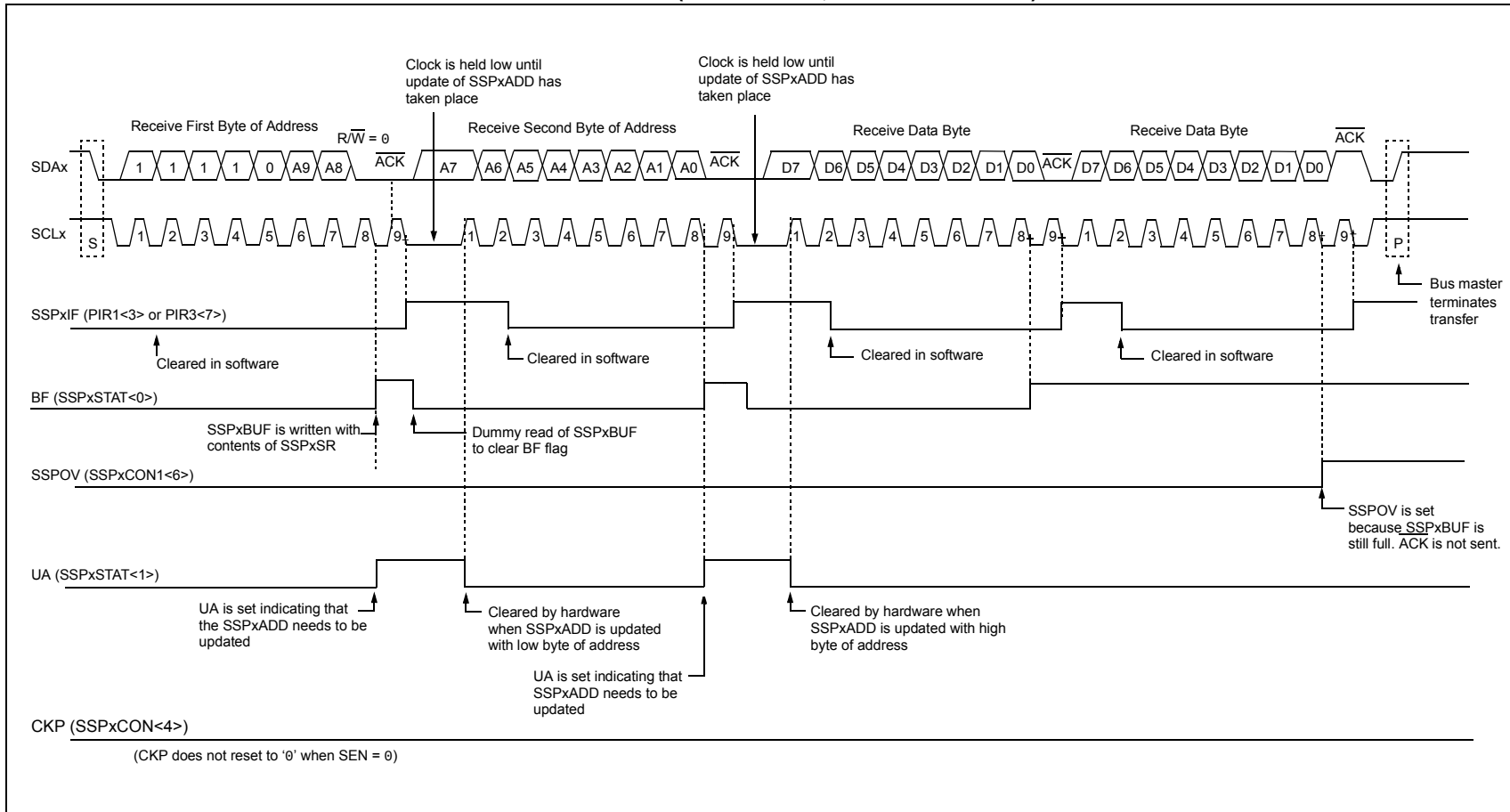
FIGURE 20-12: I 2 C SLAVE MODE TIMING WITH SEN = 0 (RECEPTION, 10-BIT ADDRESS)
