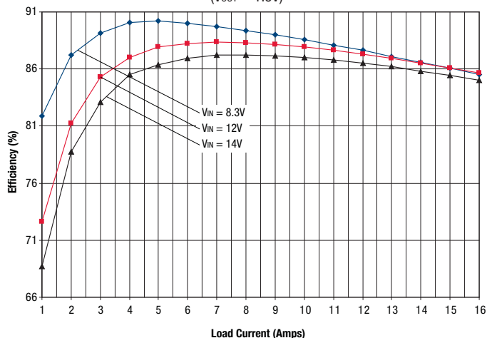
OKX2-T/16-D12 Efficiency vs. Line Voltage and Load Current @ +25°C (V OUT = 1.5V)
