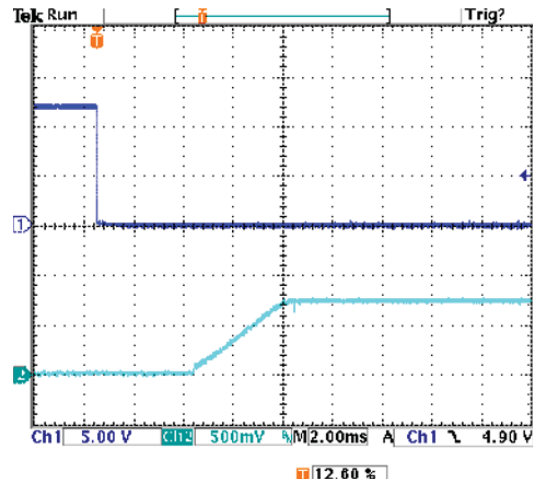
OKX2-T/16-D12-C On/Off Enable Startup Delay ( V_{IN}=12V , V_{OUT}=0.75V , I_{OUT}=16A , C_{IN}=1000\mu F , C_{LOAD}=1\mu F // 10\mu F ) Trace 1=Enable In, Trace 2=Vout
