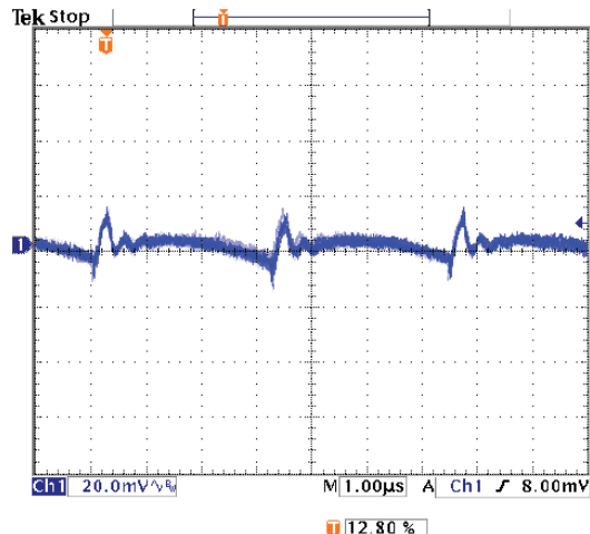
OKX2-T/16-D12 Output Ripple and Noise ( V_{IN}=12V , V_{OUT}=0.75V , I_{OUT}=16A , C_{IN}=1000\mu F , C_{LOAD}=1\mu F // 10\mu F , ScopeBW=100MHz)
