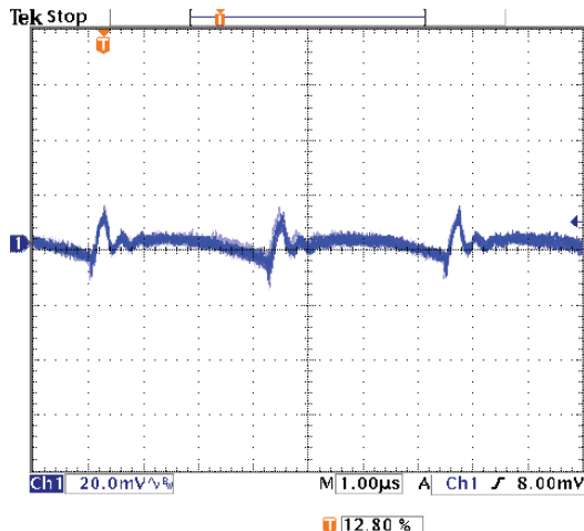
OKX2-T/16-D12 Output Ripple and Noise (V IN =12V, V OUT =0.75V, I OUT =16A, C IN =1000μF, C LOAD =1μF // 10μF, ScopeBW=100MHz)
