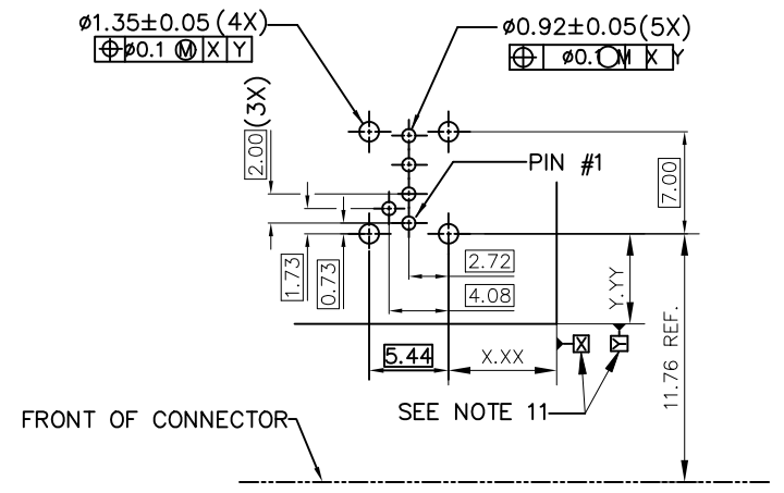
PC BOARD MOUNTING DIMENSIONS FOR 5 PIN
