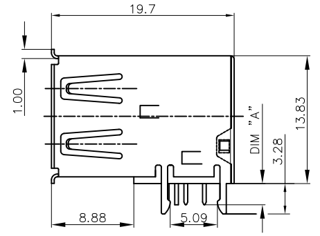
FOR 73725-X0X0B HOLD DOWN STYLE "A"
