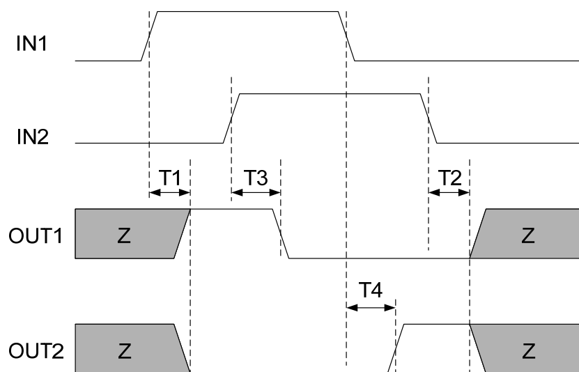
Figure 1: Input/Output Timing
