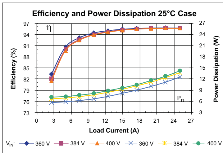
Figure 5 — Efficiency and power dissipation at T_C = 25\text{ }^\circ\text{C}
