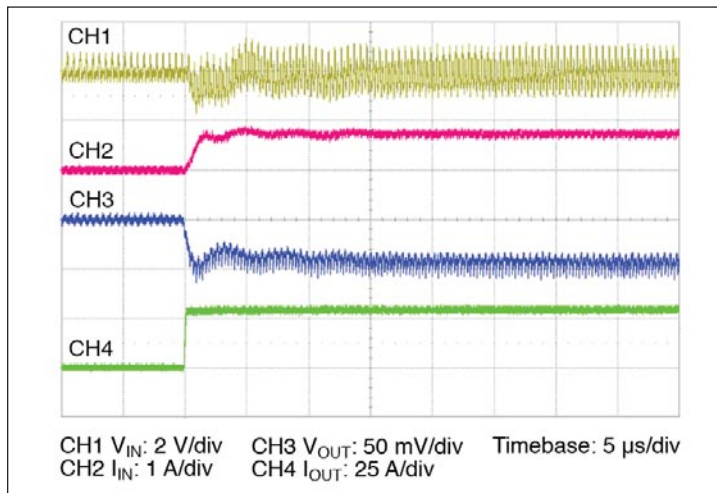
Figure 11 — 0 A – 27.3 A transient response: C_{IN} = 1 \mu F , no external C_{OUT}
