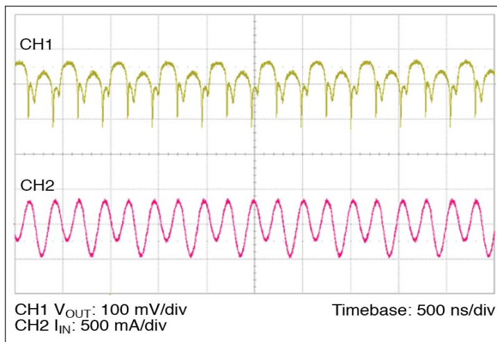
Figure 9 — Full load ripple, 1 \mu F C_{IN} ; No external C_{OUT} . Board mounted module, scope setting : 20 MHz analog BW
