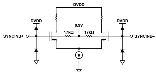
Figure 25. Equivalent SYNCINB \pm Input Circuit
