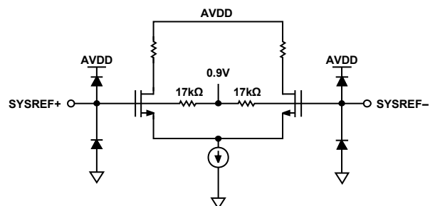
Figure 26. Equivalent SYSREF \pm Input Circuit
