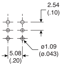
P.C. Mounting
