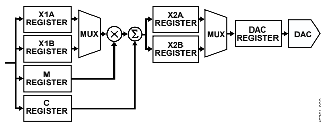
Figure 21. Data Registers Associated with Each DAC Channel
