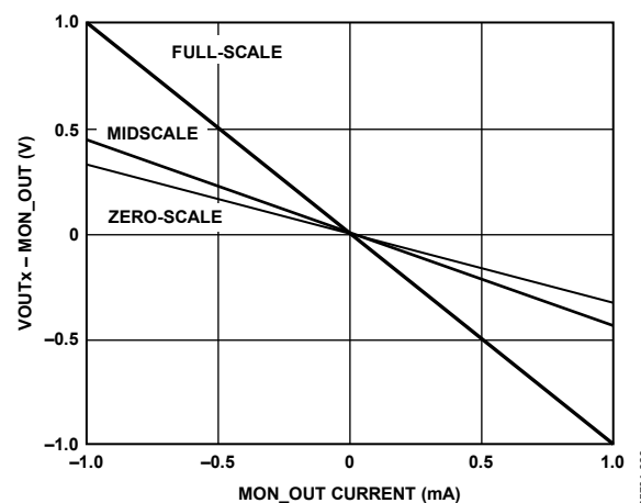
Figure 20. (V_{OUTx} - MON\_OUT \text{ Voltage}) vs. MON\_OUT \text{ Current}
