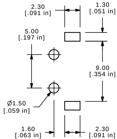
P.C. MOUNTING
