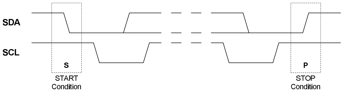
Figure 20-3. START and STOP Conditions
