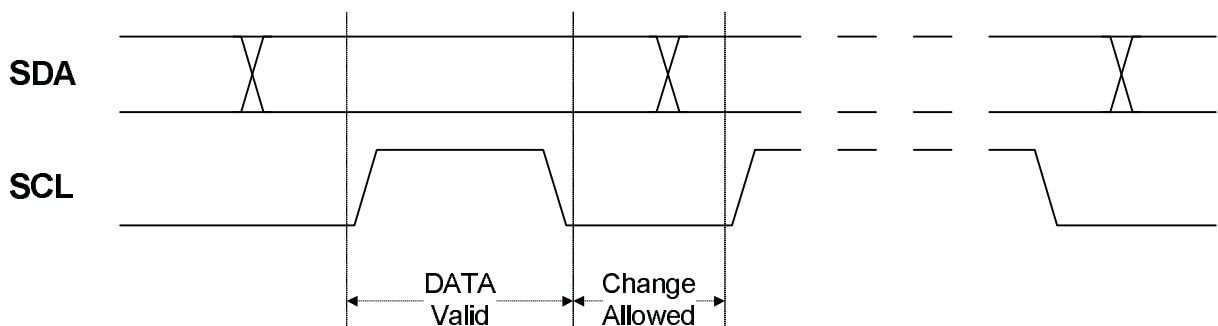
Figure 20-4. Data Validity
