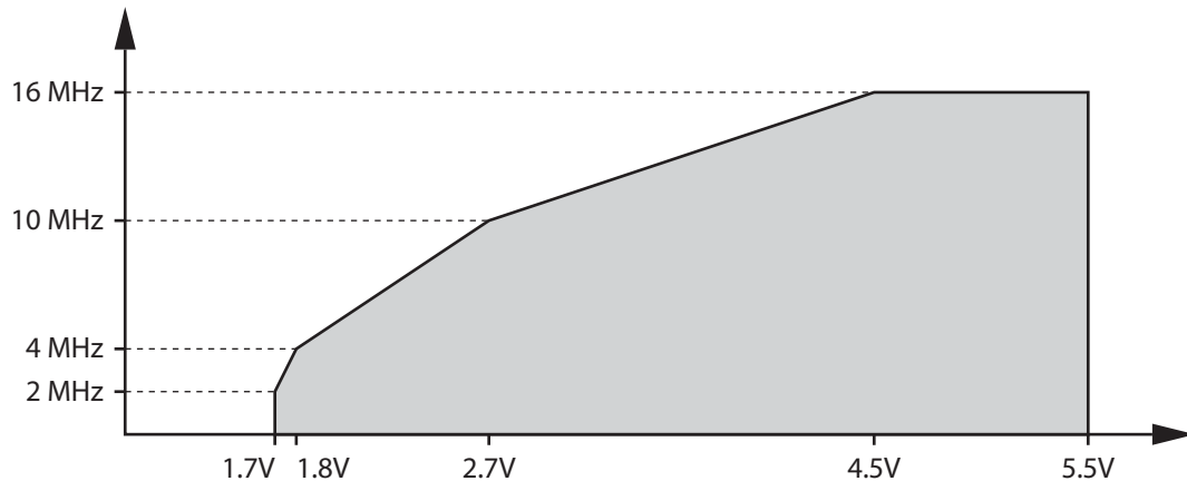
Figure 25-1. Maximum Operating Frequency vs. Supply Voltage
