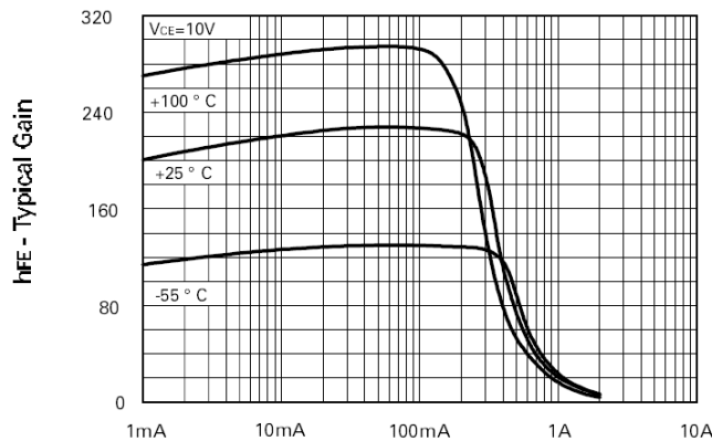
I_C -Collector Current h_{FE} v I_C
