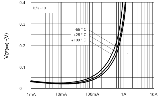
I_C -Collector Current V_{CE(sat)} v I_C
