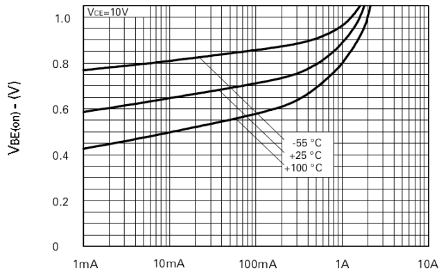
I_C -Collector Current V_{BE(on)} v I_C
