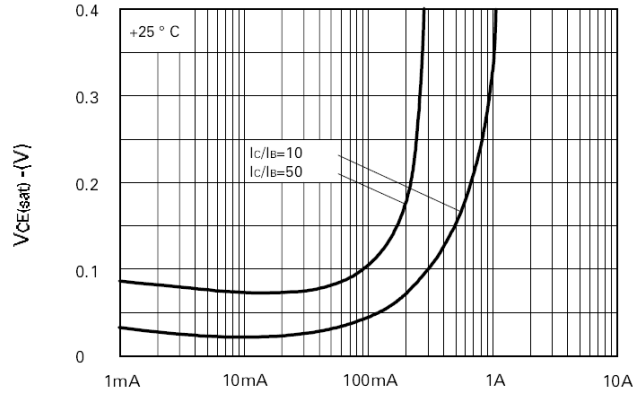
I_C -Collector Current V_{CE(sat)} v I_C
