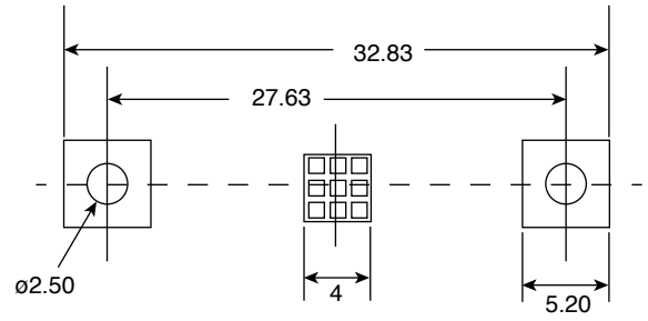
PBC Mounting Layout
