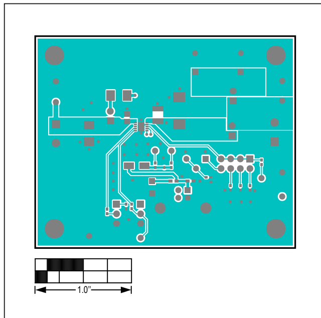
MAX17612C EV Kit PCB Layout—Top Layer
