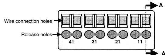
Fig. 2 Wire Connection Holes and Release Holes
