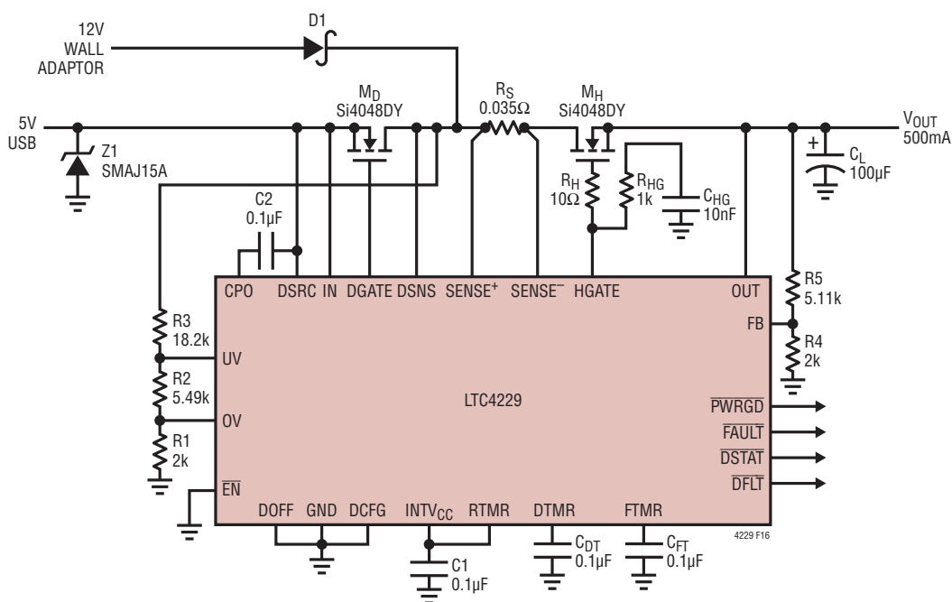
Figure 16. USB Power Combined with Wall Adaptor
