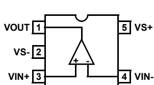
EL5111 (5 LD TSOT) TOP VIEW
