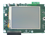
Multimedia Expansion Board (DM320005) (Includes Solomon Systech SSD1926 Controller)
