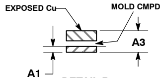
DETAIL B OPTIONAL CONSTRUCTION
