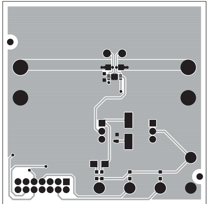
Component Side
