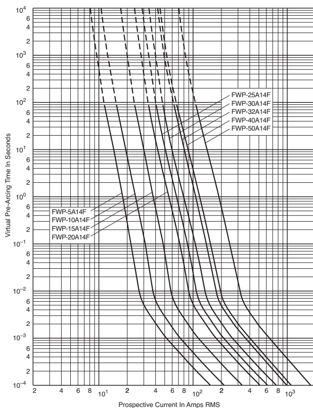
Time-Current Curve
