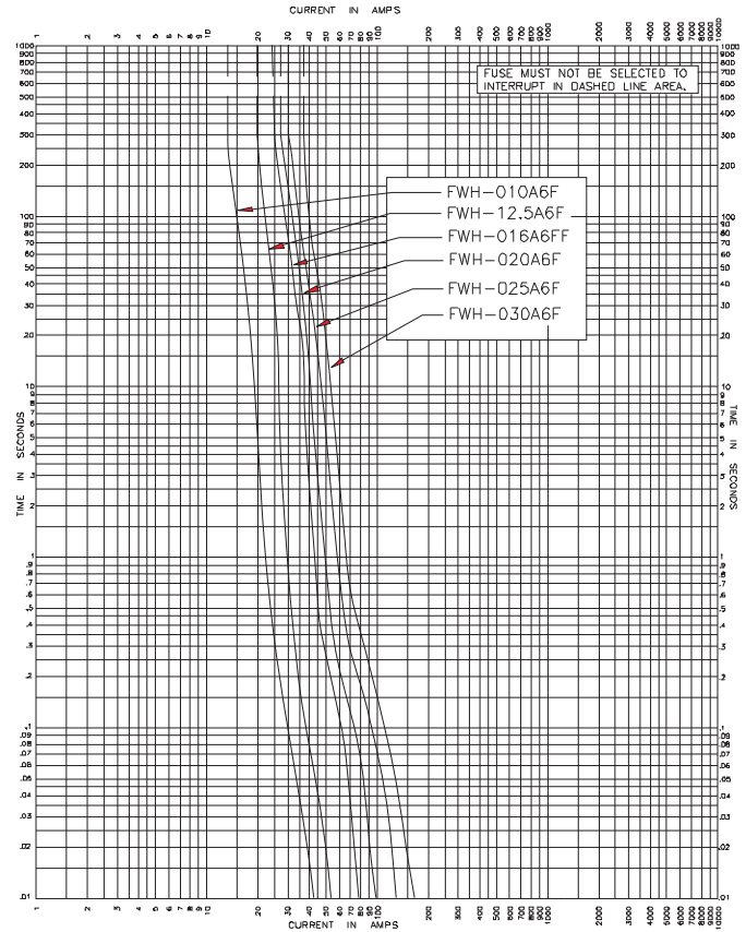
Time-Current Curve
