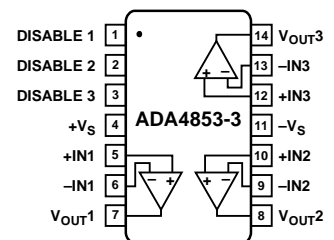
Figure 4. 14-Lead TSSOP
