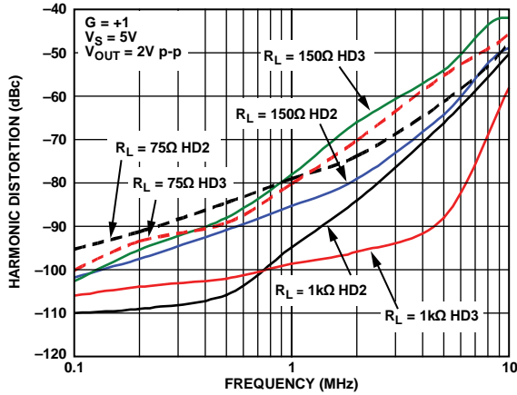
Figure 25. Harmonic Distortion vs. Frequency
