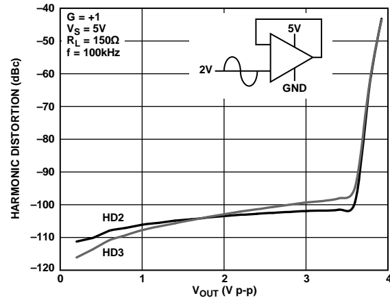
Figure 27. Harmonic Distortion for Various Output Voltages
